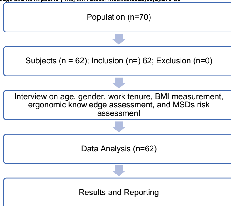
Figure 1. Research Flowchart
