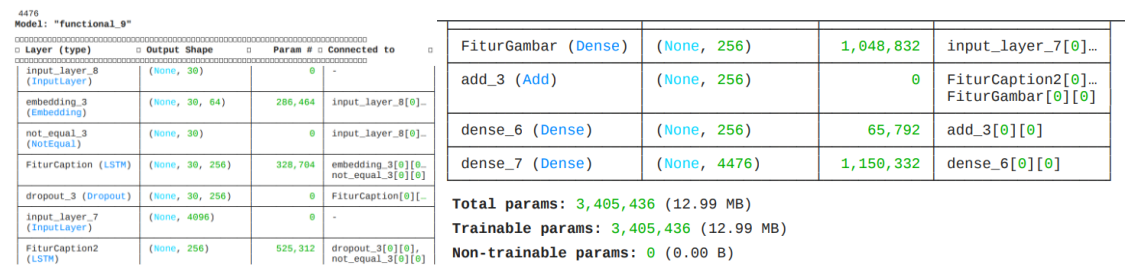
Gambar 10. Membangun Model LSTM
