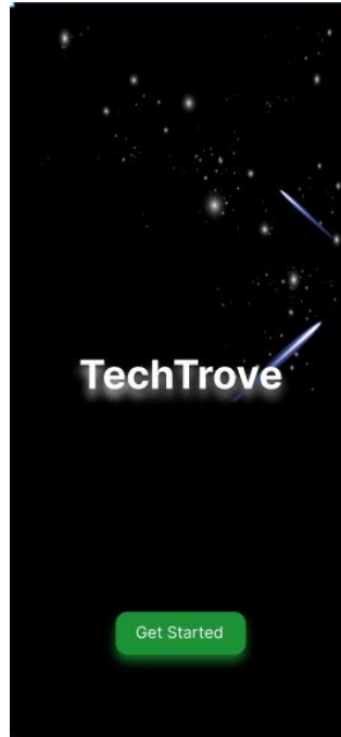
Gambar 1. Screen Awal
